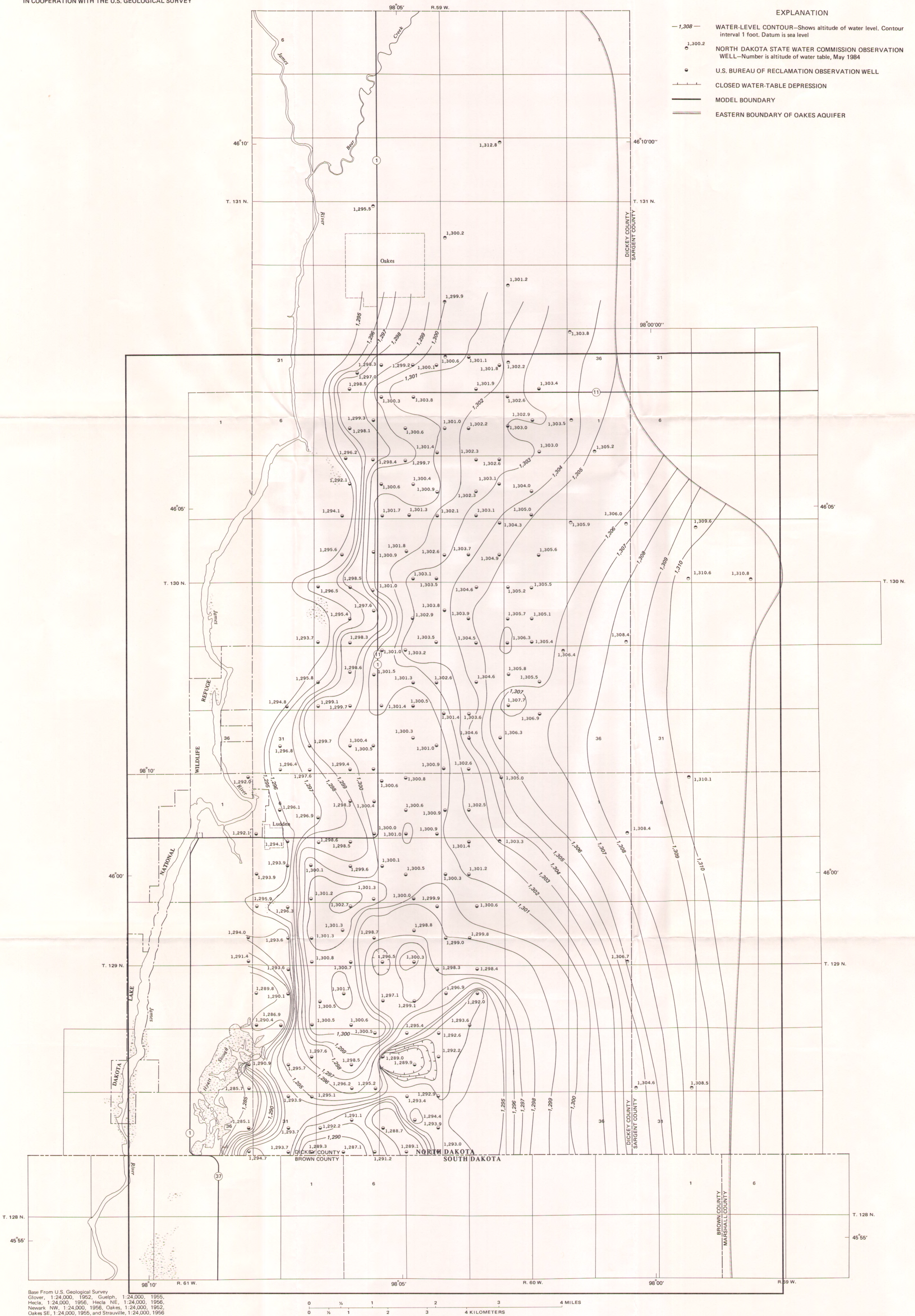
PLATE 9.—MAP SHOWING ALTITUDE OF WATER TABLE IN THE OAKES AQUIFER STUDY AREA, SOUTHEASTERN NORTH DAKOTA, MAY 1984
