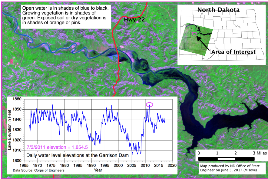
Landsat Image of the Eastern Little Missouri River Basin collected on July 3, 2011. Elevation of Lake Sakakawea (shown in the right side of Landsat image) on 7/3/2011 ~ 1,854.5 feet
