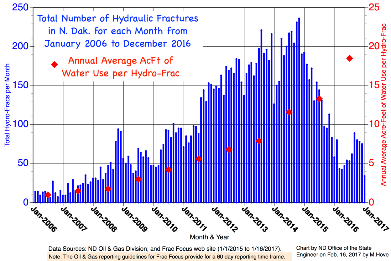
Figure C-2. Trends in the numbers of hydraulic fractures and the amount of water used per hydraulic fracture.
